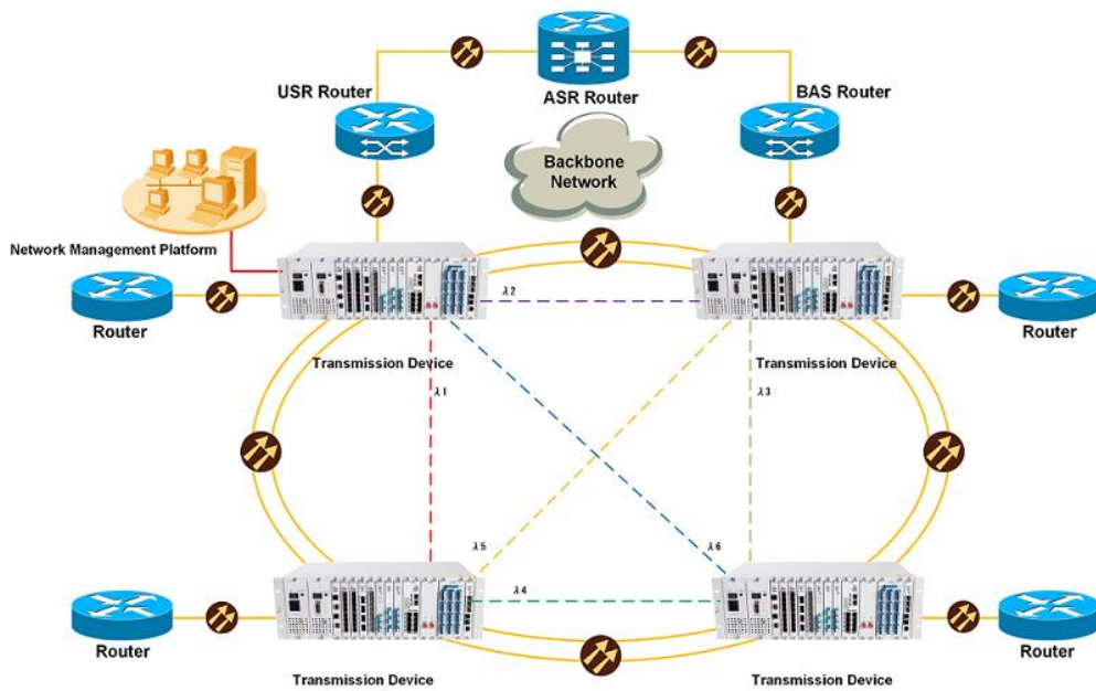
Figure 3: Ring Networking
