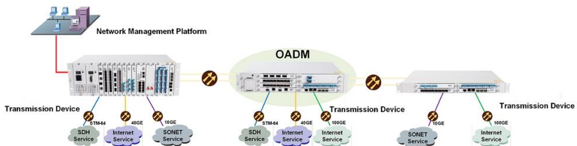
Figure 2: Chain Networking
